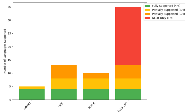
Figure 1: Languages across SLMs.
